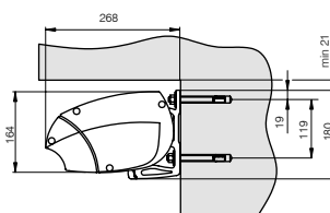
Wall/face mounting
